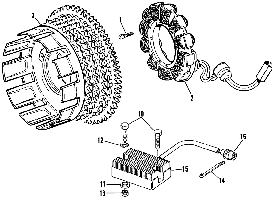
ALTERNATOR AND REGULATOR
