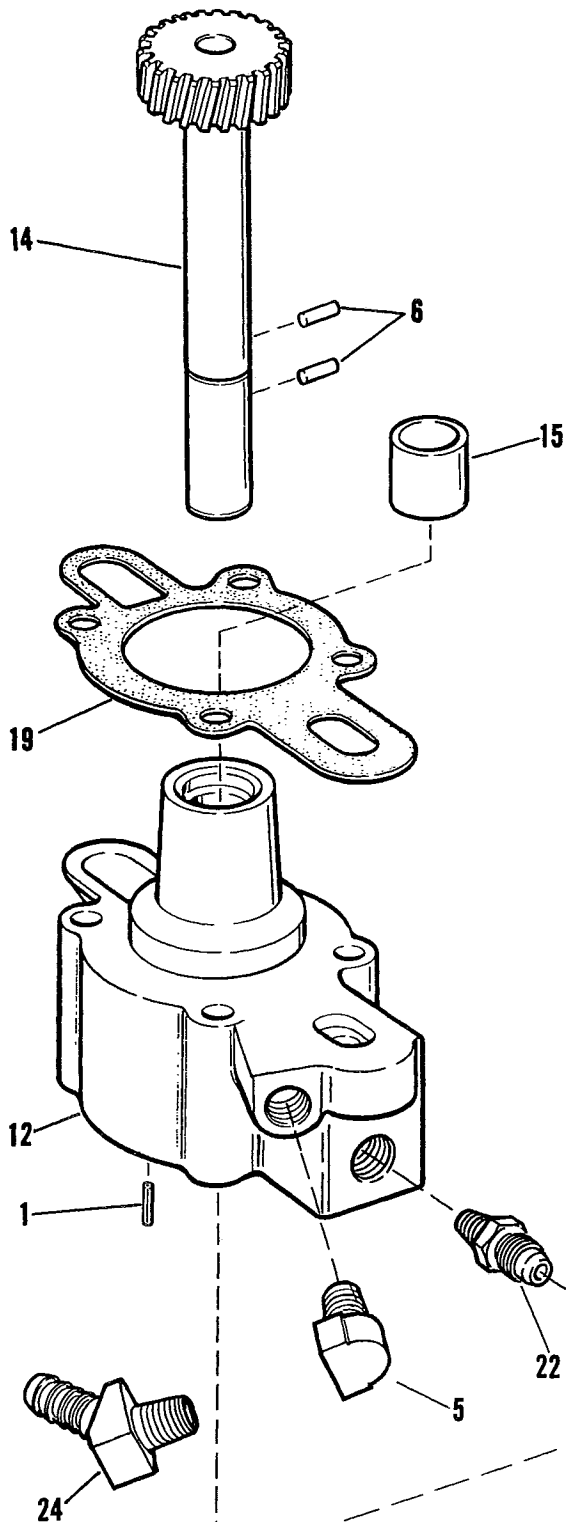
OIL PUMP
