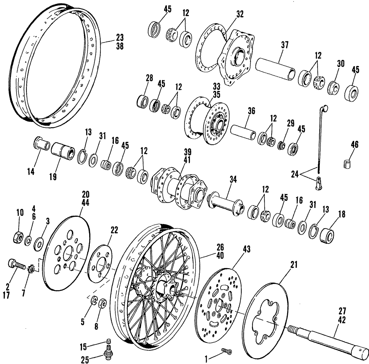
SPOKE WHEEL — FRONT 1973 & LATER
