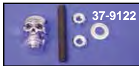
Chrome Dash Mount Stud Kit includes stud, nuts, nylon washer and either skull or acorn nut kit. Fits 1968-up cast dash panels on FXST-FL-FXWG when choke cable is not used.
