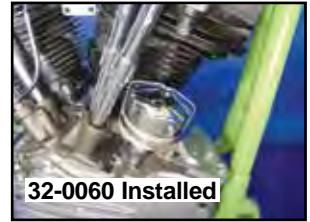
Replica 1936-47 Complete Distributors are fully assembled with natural alloy finish base with shaft and gear installed. Top housing includes early point set with spring and condenser. Stainless advance band, chrome top and clip, base retainer and points wire.
