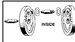
1971-99 Big Twin Bronze Inside Crank Pin Flywheel Washers sold in pairs.
