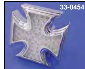
VT No. 33-0454 Wire Functions Black Wire - Ground White Wire - Running Light Orange Wire - Brake Light Red Wire - Blinker Brake Light Green Wire - Blue LED Light
