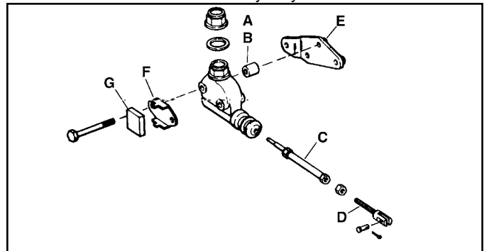
Rear Master Cylinder Hardware.
