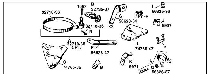
Distributor Bands, Brackets and Relay Mount.
