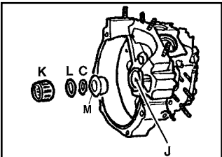
Right Crankcase Bearing and Spacers for 1958-99 Big Twin models.
